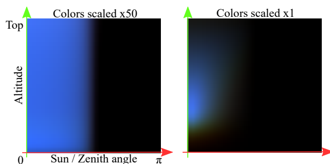
Figure 7: Visualization of Equation 10 \Psi_{ms} stored in multiple scattering LUTs. Left: the LUT for the Earth setup. It is broadly uniform, and scattering dominates over transmittance. Right: 50 times denser air, causing Rayleigh scattering with a modified distribution d^r(h) = e^{\frac{h}{20km}} . The contribution of multiple scattering increases with the density of the medium, until transmittance overtakes it, resulting in a drastic reduction of light reaching the ground. This is especially true when the sun is close to the horizon.
