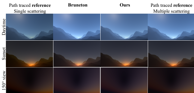
Figure 9: Rendering Earth’s atmosphere with different techniques under different conditions: daytime, sunset, and a 150 degree view of the sky with sun below the horizon revealing the shadow cast by the Earth within the atmosphere. Note: various exposures are used in this figure to ensure that visuals are readable.
