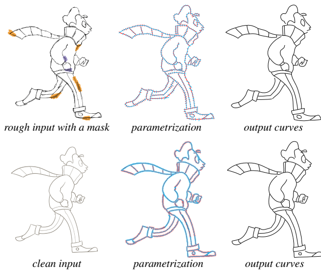
Figure 8: Using a sparse mask on the heavily over-sketched RUNNING KID (top), our vectorization is close to the one obtained using a clean version of the same input (bottom). (Purple scribbles: less simplification, orange scribbles: more simplification.)
