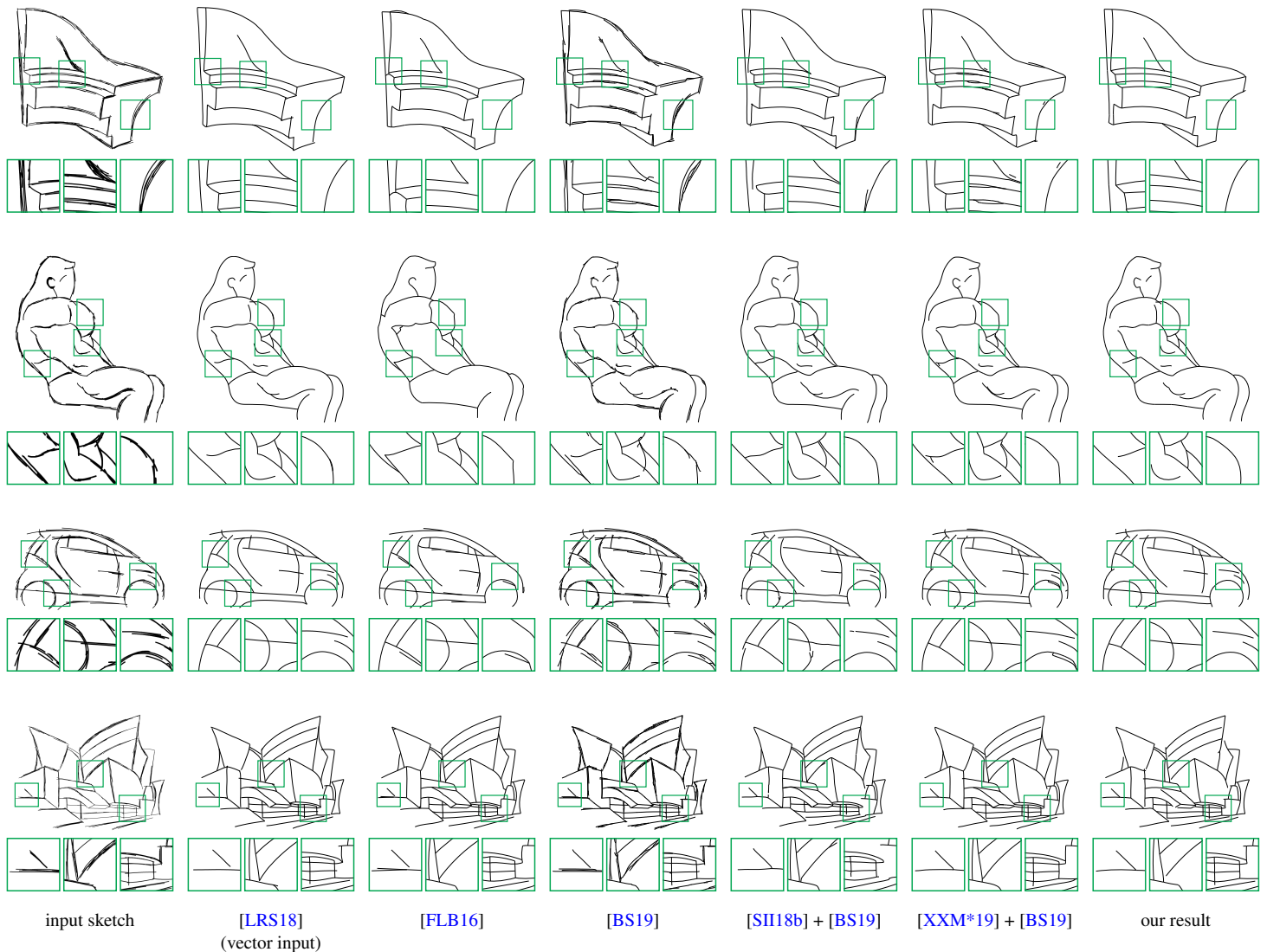
Figure 12: Results on over-sketched drawings. Our method is on par with the one by Liu et al. [LRS18], which takes vector strokes as input. Other vectorization methods [FLB16; BS19] fail to merge neighboring parallel strokes. Although bitmap filtering methods [SII18b; XXM*19] can be used to pre-process a rough input before feeding it to a vectorization algorithm, they often create artifacts. For the methods by Favreau et al. [FLB16], Simo-Serra et al. [SII18b], and Xu et al. [XXM*19] we have adjusted the parameters to obtain the best results, and we ran the method by Bessmeltsev and Solomon [BS19] with the default settings. Please see Fig. 9 for additional comparisons to vectorization methods, Fig. 10 for additional comparisons to bitmap filtering methods, and the supplemental materials for complete results.
