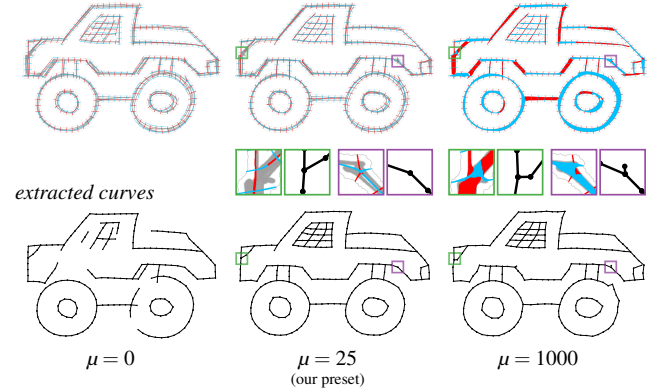
Figure 6: If the snapping term is disabled ( \mu = 0 ) the isolines fail to closely follow the input curves. Too much snapping ( \mu = 1000 ) creates degeneracies in the parametrization. We use \mu = 25 to balance these two extremes.
