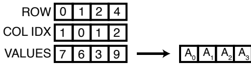
Figure 1: Prior to symbolic execution, we transform the values array of the CSR matrix A to contain symbolic entries corresponding to the location in the array.
