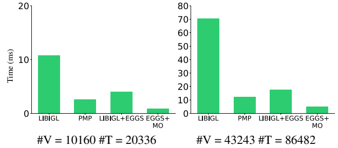
Figure 13: Additional manual optimizations (EGGS + MO) can further reduce the running time.
