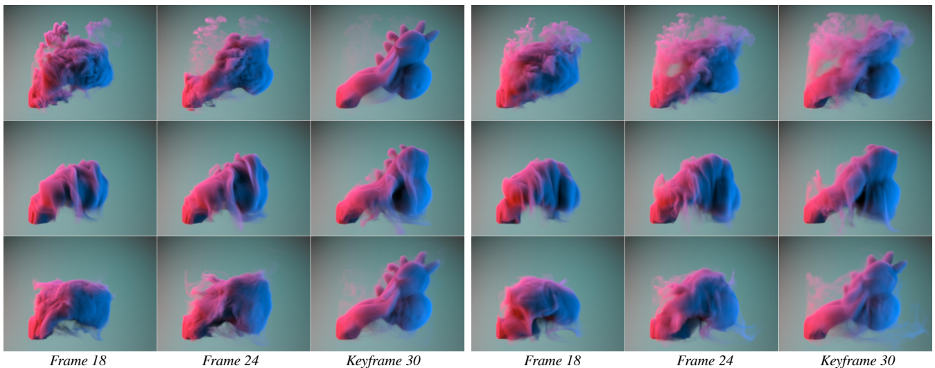
Figure 15: 3D toy example at resolution 128^3 using methods of Baseline (top row), Baseline w/TV (middle row) and Ours (bottom row). A pre-defined rubber toy shape is used as a target. The method of Baseline creates density sinks to match the target keyframe by exploiting the numerical dissipation of Euler integrator (left three columns), but fails to match the target keyframe when 3 rd order Runge-Kutta integrator is used (right three columns). The method of Baseline w/TV prevents the density sinks but fail to match the target keyframe. Our method generates smooth transitions and matches the keyframe target well under both integrator schemes.
