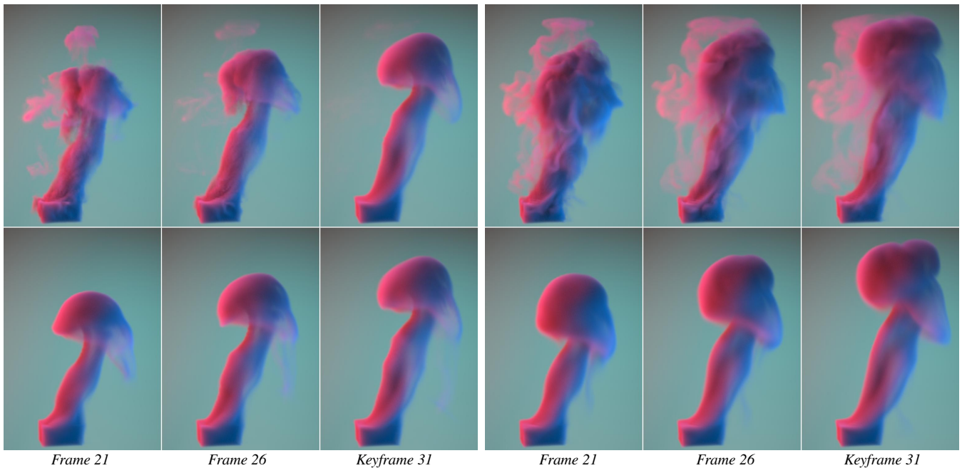
Figure 14: 3D uniform force example at resolution 128^3 using methods of Baseline (top row) and Ours (bottom row). The method of Baseline creates density sinks to match the target keyframe by exploiting the numerical dissipation of a first order Euler integrator (left three columns), but fails to match the target keyframe when 3 rd order Runge-Kutta integrator is used (right three columns). Our method generates smooth transitions and matches the keyframe target well under both integrator schemes.
