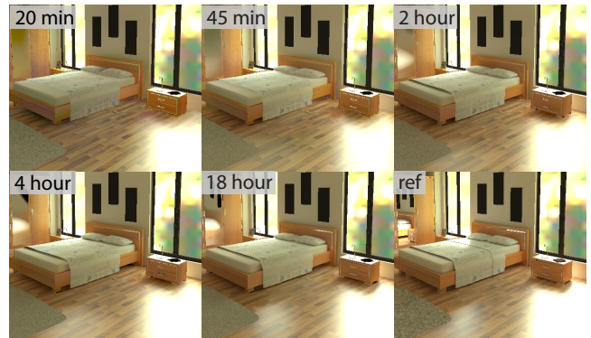
Figure 6: Prediction quality (Diffuse-Specular architecture) during training. Note the progressive appearance of the second (left) reflection of the window on the wooden floor. Scene: BEDROOM.
