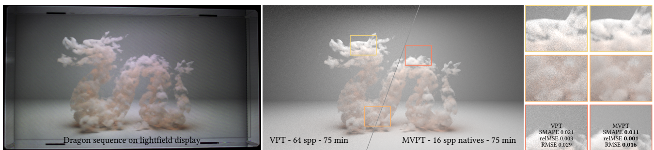
Figure 1: We render a sequence of 45 frames of the Dragon cloud scene including heterogeneous medium to be displayed on a lightfield screen. Instead of rendering the sequence frame by frame using volumetric path tracing (VPT), our method (MVPT) jointly renders the sequence at once reusing some computation during the simulation. We observe a significant variance reduction at equal time when rendering the whole sequence – or reach a desired quality at lower time. In addition the correlation of reused paths between nearby frames almost makes the flickering caused by dissimilar random sampling disappear. This makes the sequences pleasier to the eye even at low sample count.
