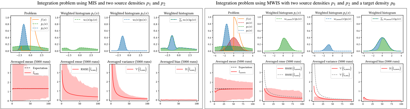
Figure 3: Difference between MIS (left) and MWIS (right) to integrate f , shown in orange, using two distributions p_1 and p_2 . Given an a-priori distribution p_0 (red) that better fits the integrand, MWIS reweights samples such that the weighted sample histogram perfectly reproduce the target density p_0 . This results in a reduction of the error and variance, at the expense of a slight bias that vanishes in O(n^{-1}) . We exploit MWIS to reweight shifted samples as if they were directly sampled from the pixel they contribute to.
