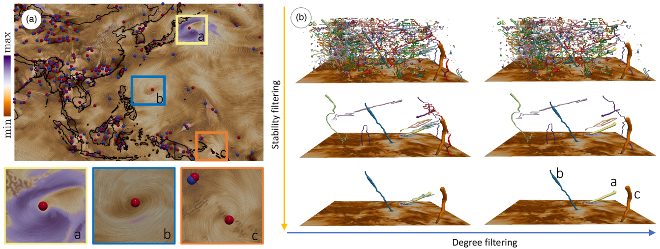
Figure 10: Feature tracking and selection for the E3SM Wind L dataset. (a) A selected vector field with zoomed-in views, where saddles are in blue, and critical points with degree +1 are in red. (b) Tracking results with degree filter thresholds at -1 and -0.2 (from left to right) and stability filter thresholds at 0 , 0.2 and 0.4 (from top to bottom).
