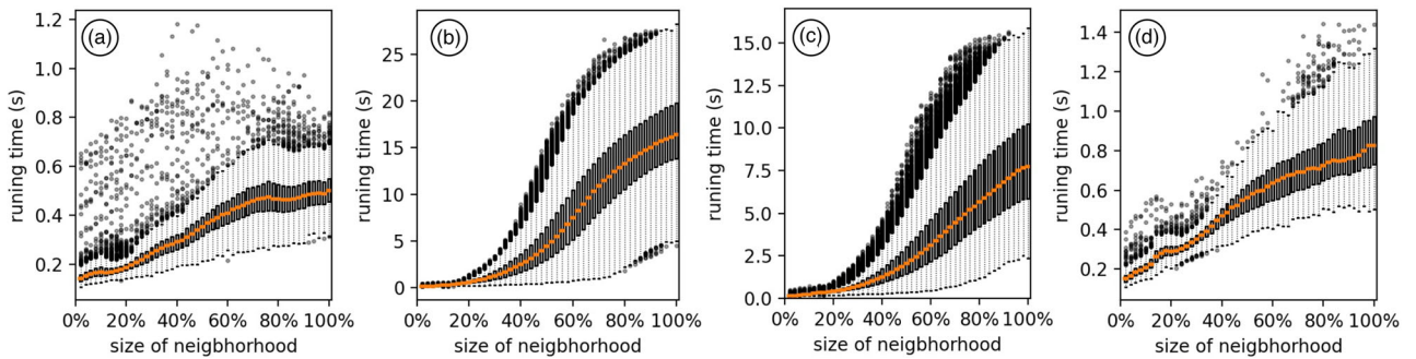
Figure 9: Boxplots of running time with different neighbourhood sizes for the (a) E3SM Wind, (b) E3SM Wind L, (c) Hurricane Katrina and (d) MPAS O Eddy datasets.
