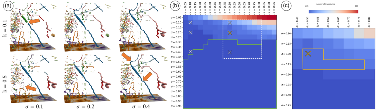
Figure 7: Parameter selection of k and \sigma for the E3SM Wind dataset. (a) From top to bottom, feature tracking results for k = 0.1 and 0.5 . From left to right, \sigma = 0.1 , and 0.4 . (b) Number of trajectories w.r.t. parameter selection of k and \sigma . (c) A zoomed-in view of (b) for the region surrounded by the dashed white box.
