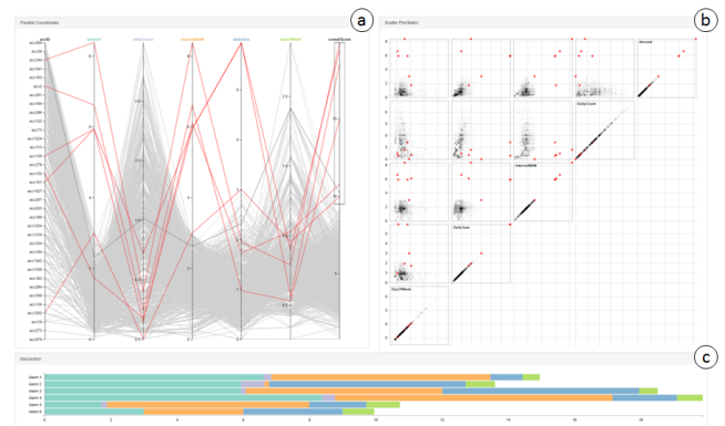
Figure 1: Filter and selection interactions linking parallel coordinates (a), scatter plots (b), and horizontal stacked bar charts (c).
