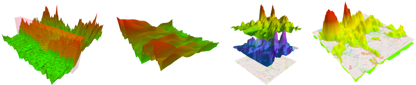
Figure 1: Heightmaps in VR. We investigate the design space of VR heightmaps, discuss interaction techniques, such as interactive color adaptation, selection (left), and zooming/filtering (center left). The overall focus is set on comparative heightmap visualizations. We use a stacked multi-layer design (center right) and enable the user to interactively position layers of heightmaps (right).
