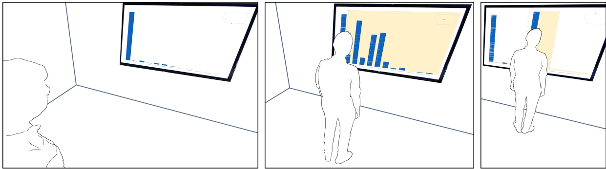
Figure 2: Prototype 2: Dynamic Scaling. This prototype uses distance and position to re-scale elements. The implicit zone (left) provides a general overview of the data with a single scale. In the subtle zone (center), the zoom scale is introduced to help people compare the rest of the bars to the extreme value. In the personal zone (right), the zoom scale is only applied to the bar in front of the user.
