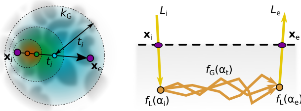
Figure 3: Left: Aggregation of the material parameters, using three color-coded Gaussians (see Eq. 1). Right: Decomposition of the transport kernel into local and global components f_L and f_G (see Eq. 2).
