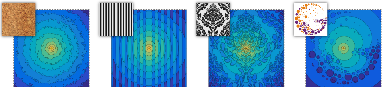
Figure 1: Predictions of the spatially varying sub-surface scattering kernels (false-color logarithmic maps) for heterogeneous materials (defined by 2.5D scattering albedo textures shown in the respective thumbnails). The proposed framework consists of two key steps: 1) a principled statistical aggregation of the material properties, and 2) a suitable decomposition of the sub-surface scattering kernel in order to preserve both the local and global illumination features.
