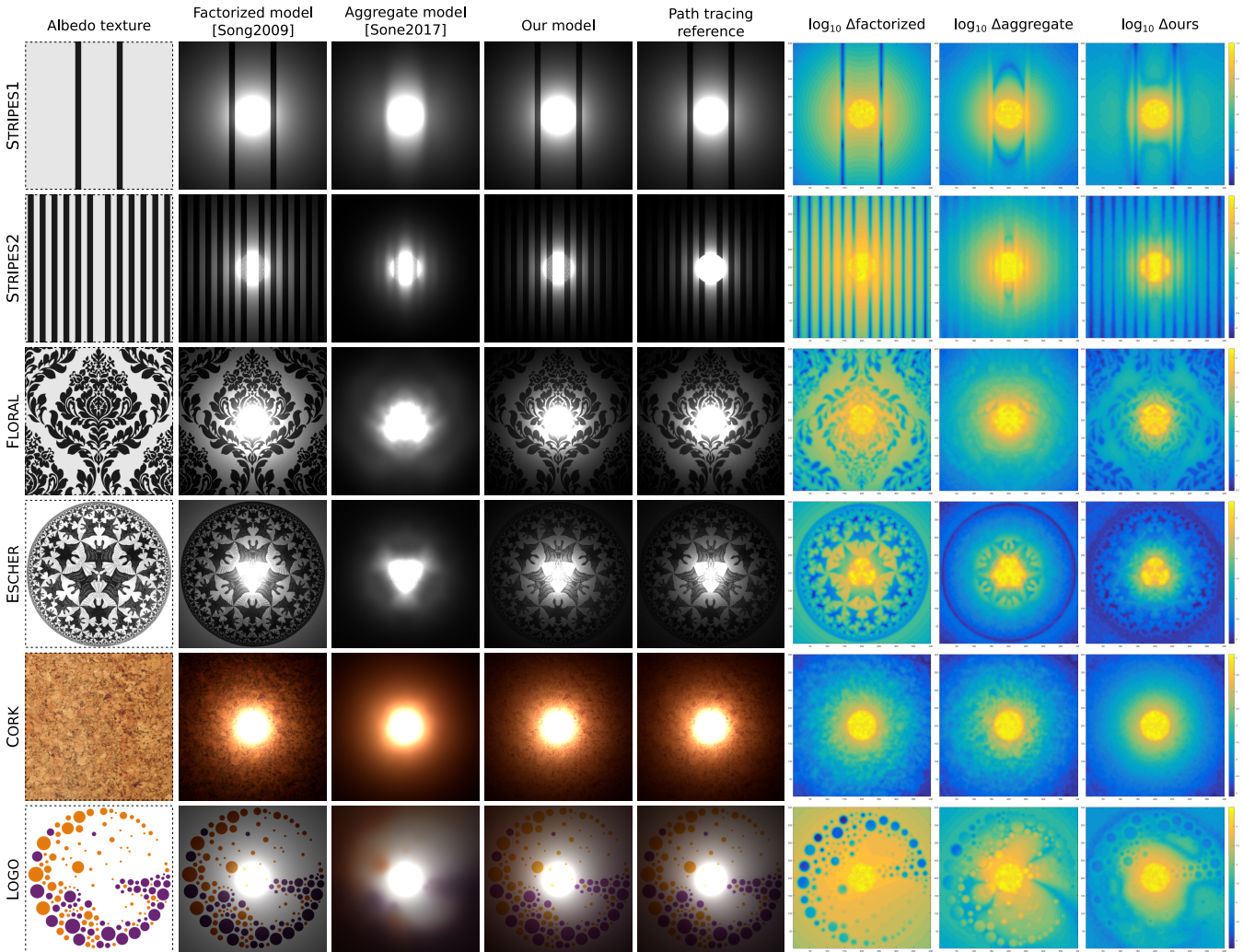
Figure 4: Main evaluation of the proposed method, discussed in Sec. 3. The renders are tone-mapped with the standard Gamma operator and manually exposed to emphasize the indirect sub-surface transport. The false-color plots show the absolute difference from the reference, and were blurred with a small Gaussian kernel to eliminate spike noise in the visualization.
