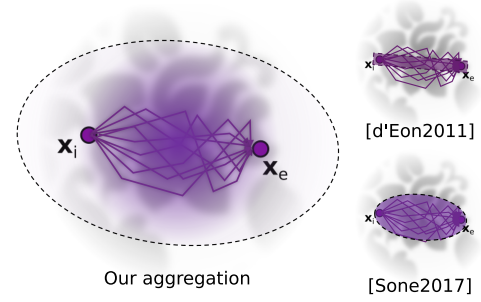
Figure 2: Our framework regards the material aggregation kernel as a smooth ‘footprint’ of the sub-surface path distribution. This contrasts with the existing heuristics which perform the aggregation within an empirically bounded region, such as a line [d111] or ellipse [SHK17].
