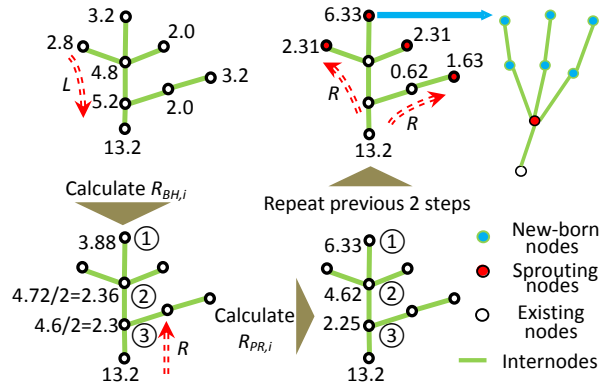
Figure 3: An illustration for resource distribution for parameters: \lambda = 0.55 , \omega_1 = 1.0 , \omega_2 = 0.6 , \omega_3 = 0.3 and an example of new-born nodes.
