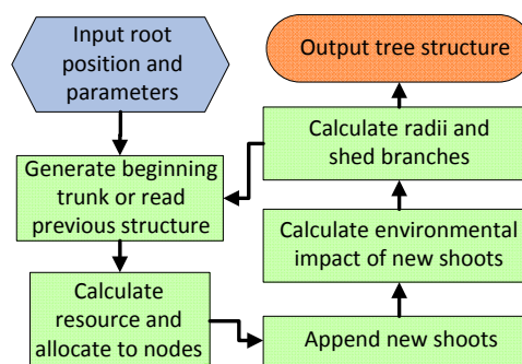
Figure 2: Overview of algorithm.
