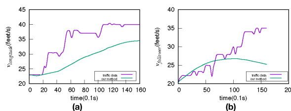
Figure 9: Comparison between a simulated result by our method and the ground-truth data. (a): The velocity of the subject vehicle in the longitude direction, and (b): the velocity of the follower vehicle. This vehicle took 178 frames to complete the lane-changing. It is obvious that the predictions are less accurate after the 85-th frame.
