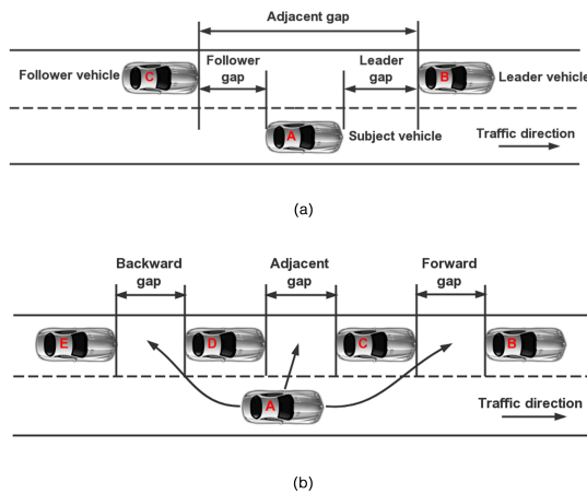
Figure 2: Schematic differences between our method and previous lane-changing models: (a) the previous methods only focus on the adjacent gap on the target lane; (b) our method also considers the forward and backward gaps, besides the adjacent gap.
