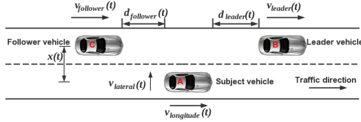
Figure 4: Schematic illustration of the input variables to the learned lane-changing execution model
