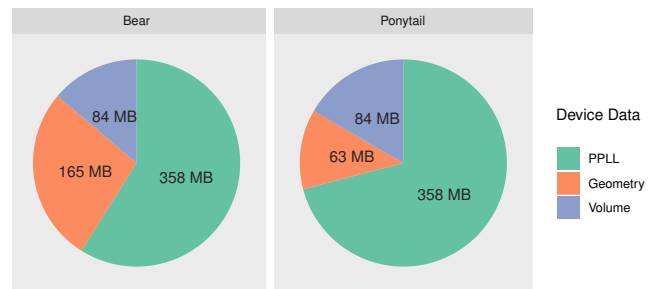
Figure 6: GPU memory usage breakdown. Our volumes don’t have to use inordinate amounts of memory when compared to its original geometry, and can be adjusted by voxelizing at lower resolutions. The primary “bottleneck” is the PPLL that’s used for transparency.
