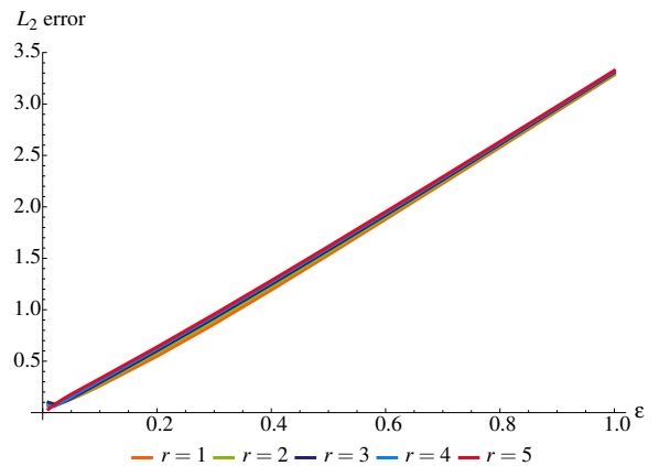
Figure 6: L_2 error between the SH BRDFs and the exponentiated log-SH BRDFs for various values of r and \epsilon .
