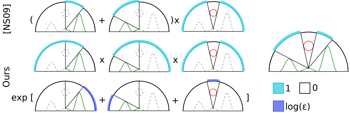
Figure 3: Combining visibilities. Top: The visibility wedges are added before we multiply them with the blockers’ visibility vectors. Middle: Adding in log-SH space is equivalent to multiplying in SH space. Bottom: When using spherical harmonics exponentiation, we add the visibility vectors in log-SH space; the numerical values are inverted as \log(1) = 0 , and we use a factor \epsilon because \log(0) is undefined. Right: The resulting visibility.
