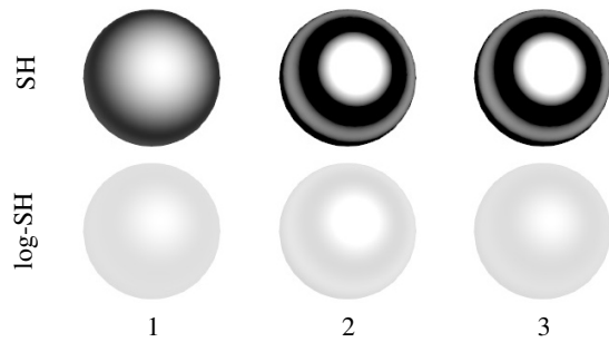
Figure 7: Spheres lit by a directional light with varying r . Our log-SH BRDF is a coarse approximation of the SH BRDF, but avoids a costly triple-product integration. Here log-SH uses \epsilon = 0.2 .
