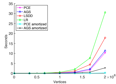
Figure 12: Computational cost associated to each gradient estimator. The amortized curves refer to the cost of matrix vector multiplication only (the matrix is assumed to be pre-computed). Our current implementation of AGS is not optimal, as gradients are evaluated per triangle using the matrix, and then averaged at vertices navigating the mesh topology. Encoding the whole computation in matrix form the performances of AGS amortized should match the ones on PCE amortized.
