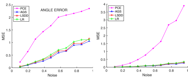
Figure 11: Plot of angle error (left) and magnitude error (right) of the four methods computed on a structured mesh, where the function sampled at its vertices was affected by increasingly high displacement to simulate noisy data. There are no significant differences between the piece-wise linear methods. The piece-wise constant method performs worse than all.
