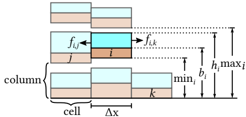
Figure 2: The simulation grid is divided into cells, which in turn contain one or more columns. Here we see three linked columns i , j , and k , and column i 's properties: its range [\min_i, \max_i] along the vertical axis, its base height b_i , and its liquid height h_i .
