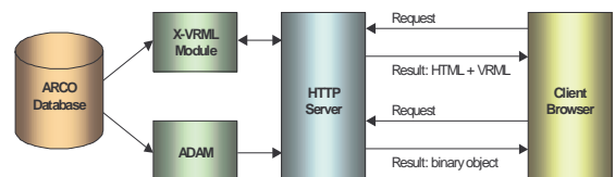
Figure 9 Architecture of the ARIF X-VRML Server
