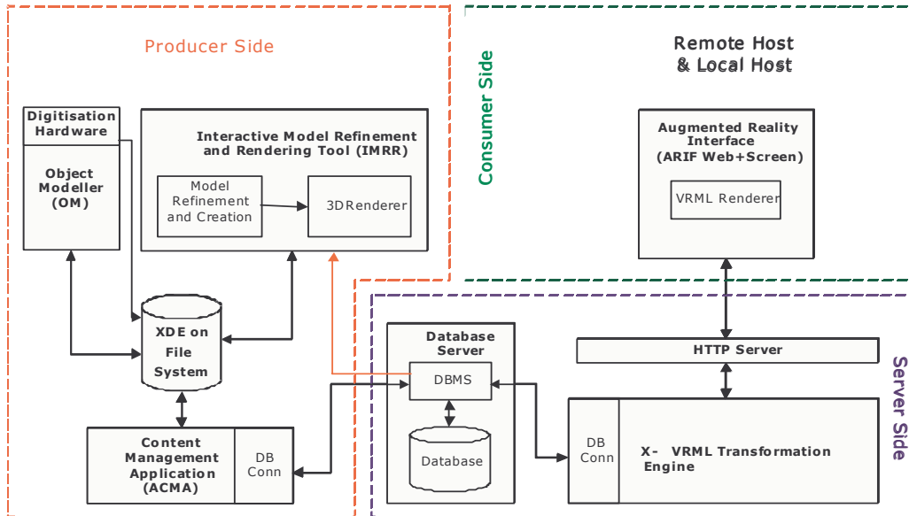
Figure 2: Major components of the ARCO system's architecture
