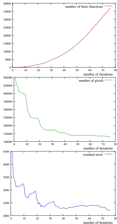
Figure 5: Behaviour of n_b the number of visual hull consistent basis functions (columns) in matrix \mathbf{S} (top), n_p the number of pixels (rows) in matrix \mathbf{S} (middle) and the residual error (bottom) versus the number of iterations of the adaptive algorithm.
