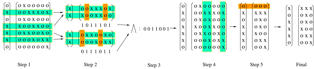
Figure 3: Visual hull restriction of matrix S .
