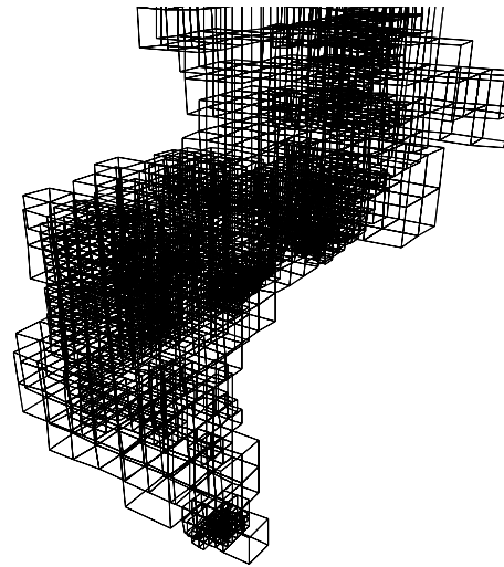
Figure 4: A visual hull restricted adaptive grid (intermediate step in the iteration).
